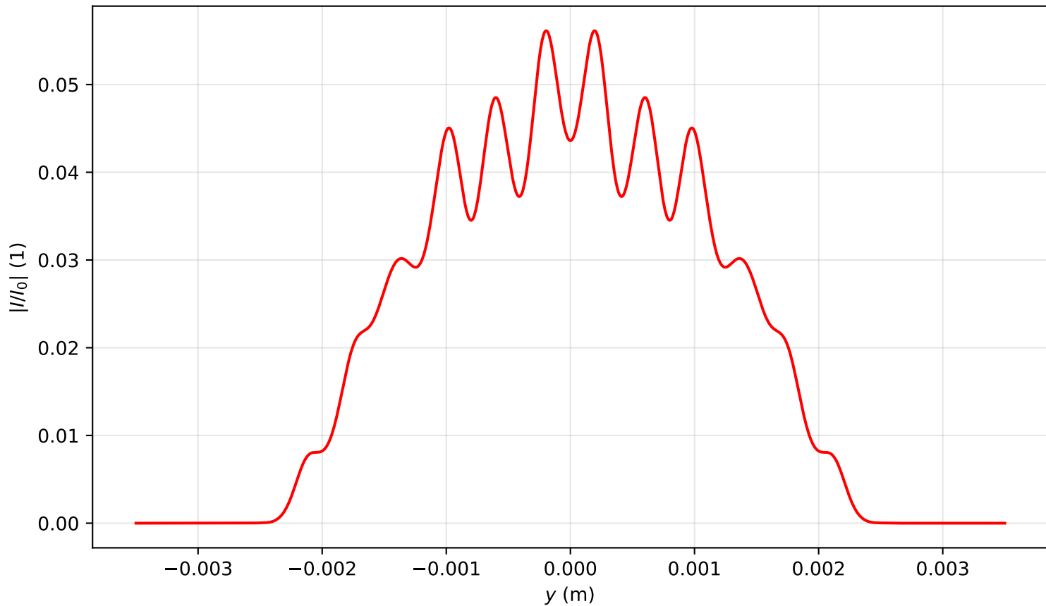
Intensity profile I(x=0, y, z=3.821)/I_0 , P_{in}=5.5P_{cr} , artificial time
